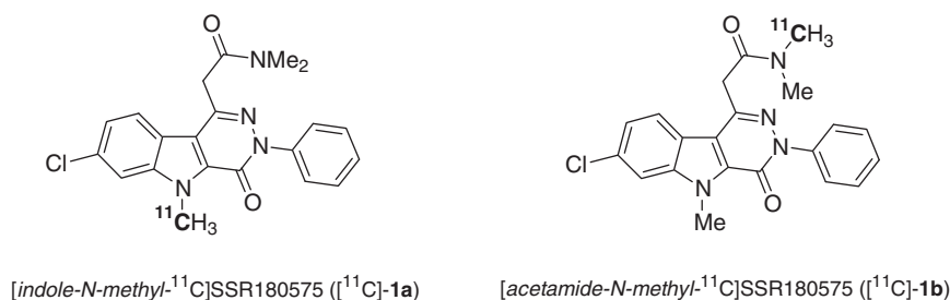
Figure 2. [ 11 C]SSR180575: chemical structures resulting from the labeling at the 5-methylpyridazino[4,5- b ]indole moiety ([ 11 C]- 1a ) and at the N,N -dimethylacetamide function ([ 11 C]- 1b ).
