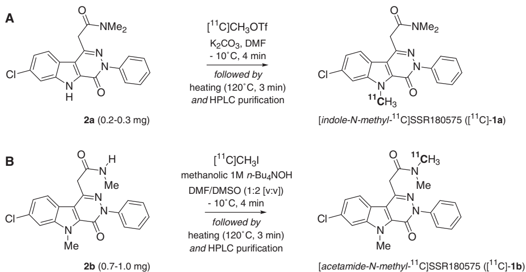
Scheme 1. Radiosynthesis of [indole- N -methyl- 11 C]SSR180575 ([ 11 C]- 1a ) and [acetamide- N -methyl- 11 C]SSR180575 ([ 11 C]- 1b ) from [ 11 C]methyl triflate and [ 11 C]methyl iodide, respectively.
